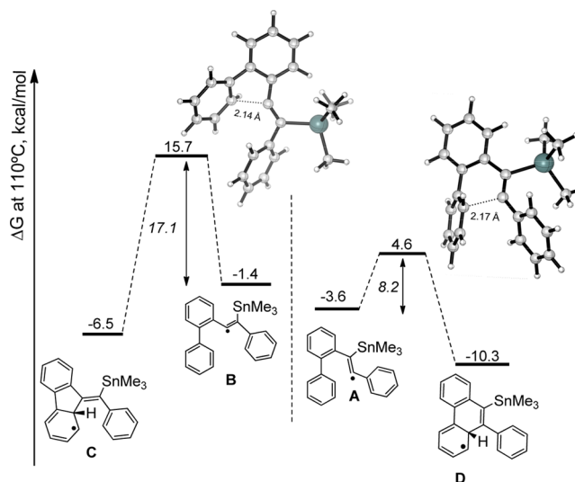
Scheme 4. Calculated Gibbs Free Energy Surface for the Sn-Radical-Mediated Transformation of Biphenyl Phenyl Alkyne at 110°C a
